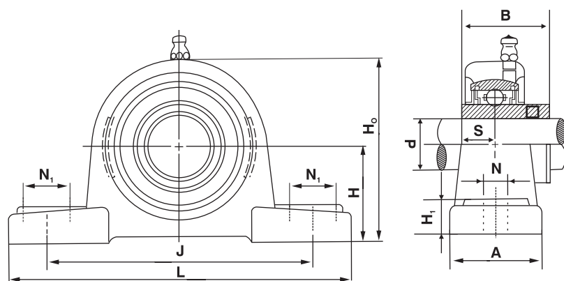
U.C.P. Technical Diagram
